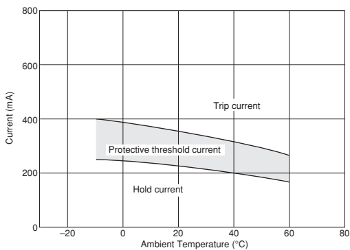
PTGL10AR150M6C61B0
