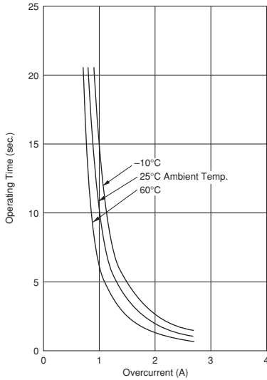
PTGL09AR4R7M3B51B0
