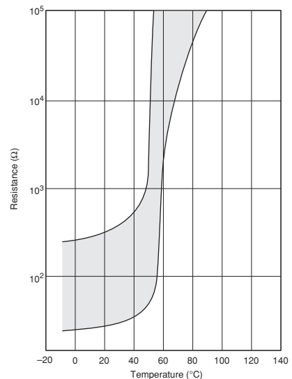
PTF_04BH222Q Type
